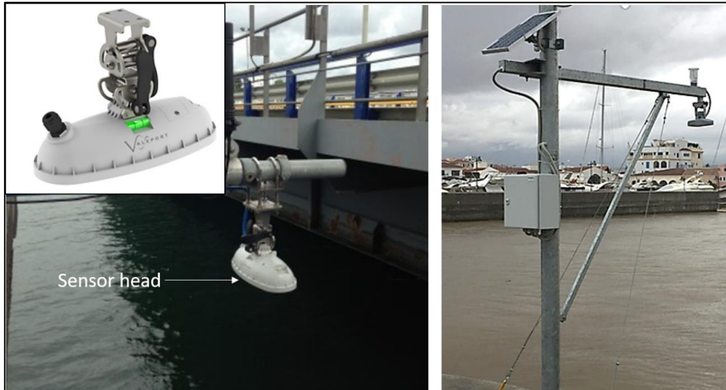
Figure 1 Radar Type Tide Gauge Installation
